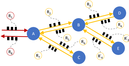
Figure 1: Call graph for an example application.
